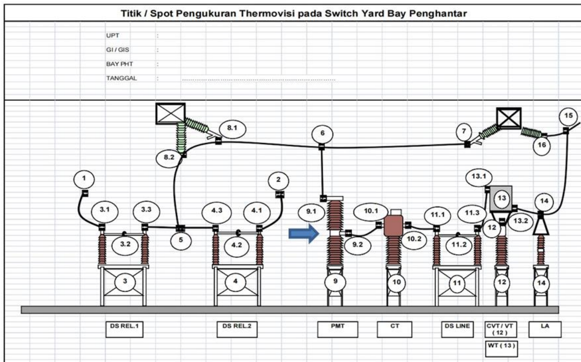
Figure 3. One Bay Conductor
