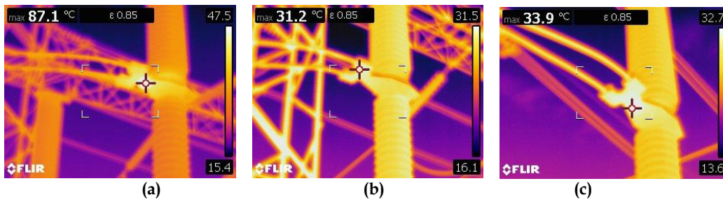
Figure 5. R, S, T phase clamps (a). Lower pole clamp CT direction Phase R (b). S-phase CT clamp the lower pole (c). Lower pole clamp CT direction Phase T
