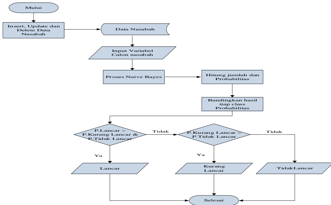
Gambar 3. Flowchart sistem
