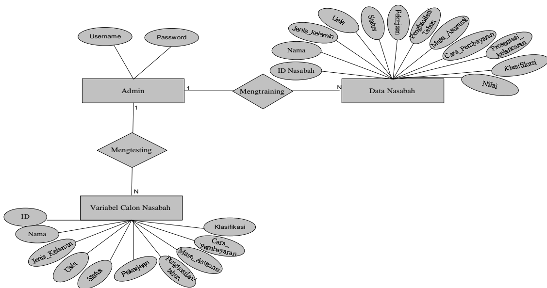
Gambar 6. Entity Relationship Diagram (ERD)
